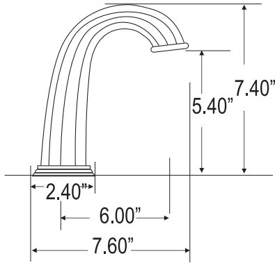
CA19 LAVATORY
