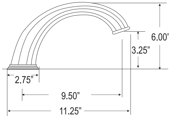
CA29 DECK
