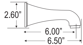
MI16 WALL MOUNT
